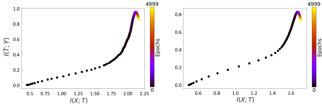
Figure 19: Effect of stochastic training in linear networks. (A) Information plane dynamics for stochastic gradient descent in a linear network (same setting as Fig. 4). (B) Information plane dynamics for batch gradient descent.
