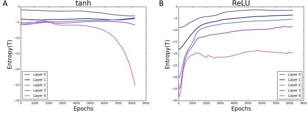
Figure 12: Entropy dynamics over training for the network architecture and training dataset of Schwartz-Ziv & Tishby (2017), estimated with the nonparametric k-nearest-neighbor-based method of Kraskov et al. (2004). Here the x-axis is epochs of training time, and the y-axis plots the entropy of the hidden representation, as calculated using nearest-neighbor distances. Note that in this setting, if T is considered to be the hidden activity plus independent noise, the entropy is equal to the mutual information up to a constant (see derivation in text). Layers 0-4 correspond to the hidden layers of size 10-7-5-4-3. (A) tanh neural network layers can show compression over the course of training. (B) ReLU neural network layers show no compression.
