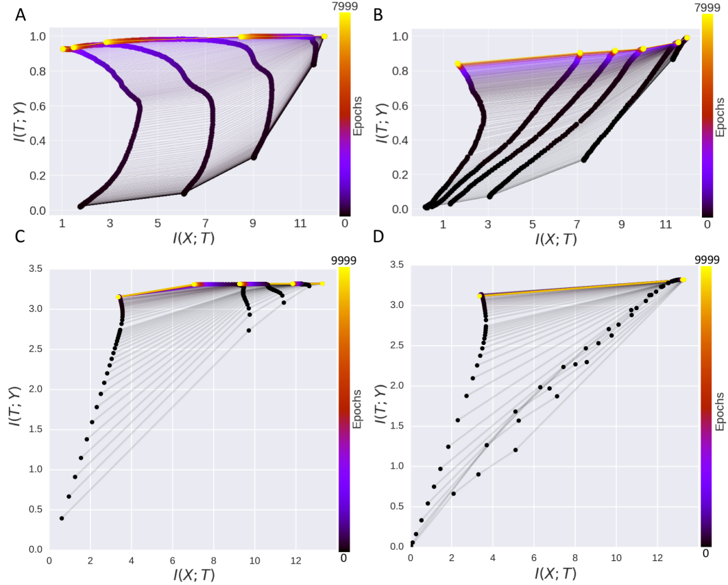
Figure 1: Information plane dynamics and neural nonlinearities. (A) Replication of Schwartz-Ziv & Tishby (2017) for a network with tanh nonlinearities (except for the final classification layer which contains two sigmoidal neurons). The x-axis plots information between each layer and the input, while the y-axis plots information between each layer and the output. The color scale indicates training time in epochs. Each of the six layers produces a curve in the information plane with the input layer at far right, output layer at the far left. Different layers at the same epoch are connected by fine lines. (B) Information plane dynamics with ReLU nonlinearities (except for the final layer of 2 sigmoidal neurons). Here no compression phase is visible in the ReLU layers. For learning curves of both networks, see Appendix A. (C) Information plane dynamics for a tanh network of size 784 - 1024 - 20 - 20 - 20 - 10 trained on MNIST, estimated using the non-parametric kernel density mutual information estimator of Kolchinsky & Tracey (2017); Kolchinsky et al. (2017), no compression is observed except in the final classification layer with sigmoidal neurons. See Appendix B for the KDE MI method applied to the original Tishby dataset; additional results using a second popular nonparametric k-NN-based method (Kraskov et al., 2004); and results for other neural nonlinearities.
