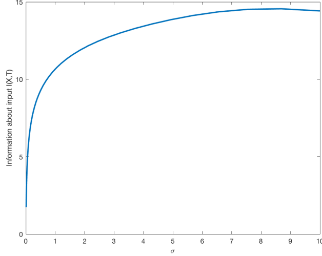
Figure 13: Effect of binning strategy on minimal three neuron model. Mutual information for the simple three neuron model shown in Fig. 2 with bin edges b_i \in \tanh(\text{linspace}(-50, 50, N)) . In contrast to linear binning, the mutual information continues to increase as weights grow.
