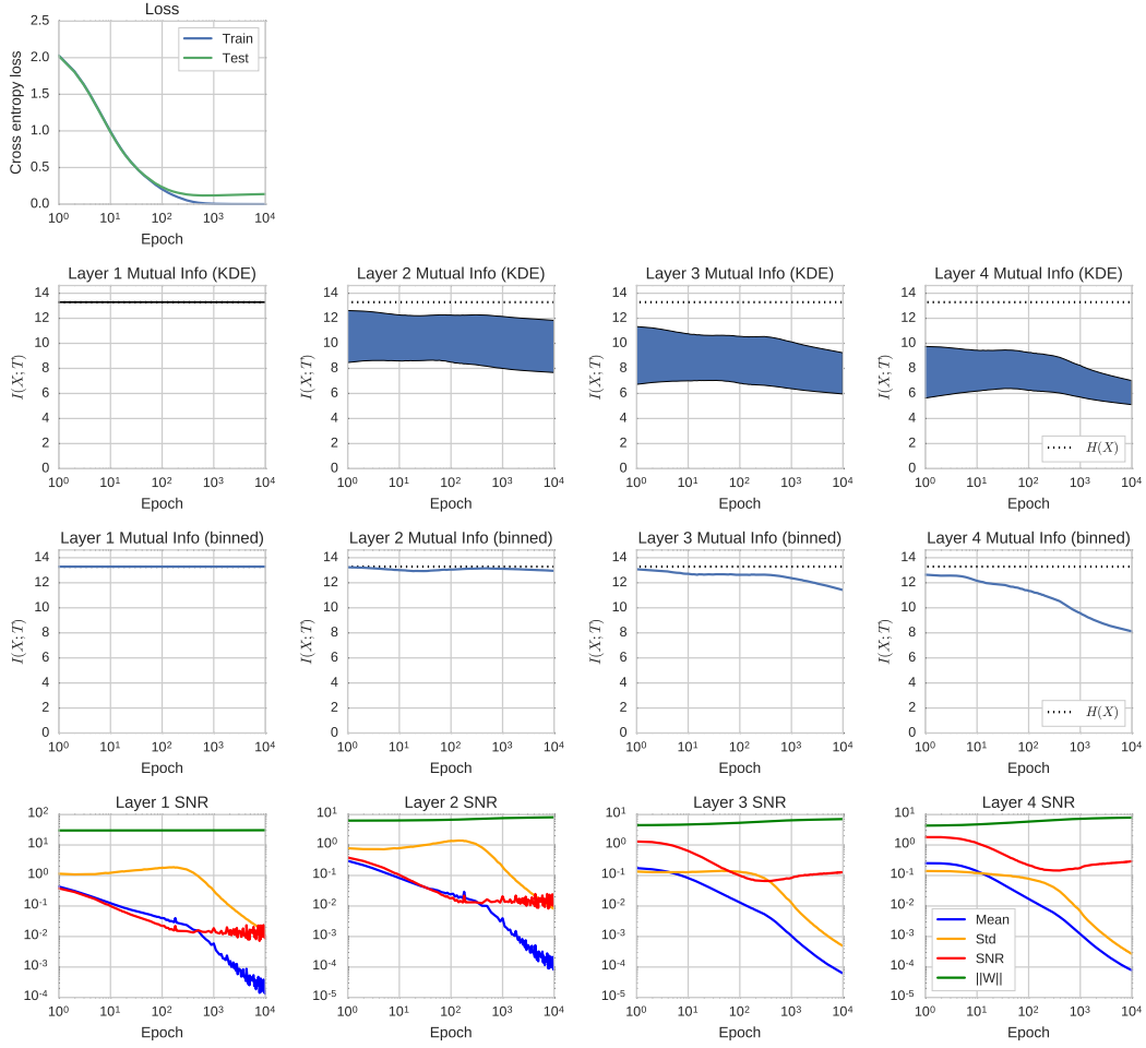
Figure 9: Detailed tanh activation function results on MNIST. Row 1: Loss over training. Row 2: Upper and lower bounds for the mutual information I(X;T) between the input ( X ) and each layer’s activity ( T ), using the nonparametric KDE estimator (Kolchinsky & Tracey, 2017; Kolchinsky et al., 2017). Dotted line indicates H(X) = \log_2 10000 , the entropy of a uniform distribution over 10,000 testing samples. Row 3: Binning-based estimate of the mutual information I(X;T) , with each neuron’s activity discretized using a bin size of 0.5. Row 4: Gradient SNR and weight norm dynamics. The gradient SNR shows a phase transition during training, and the norm of the weights in each layer increases.
