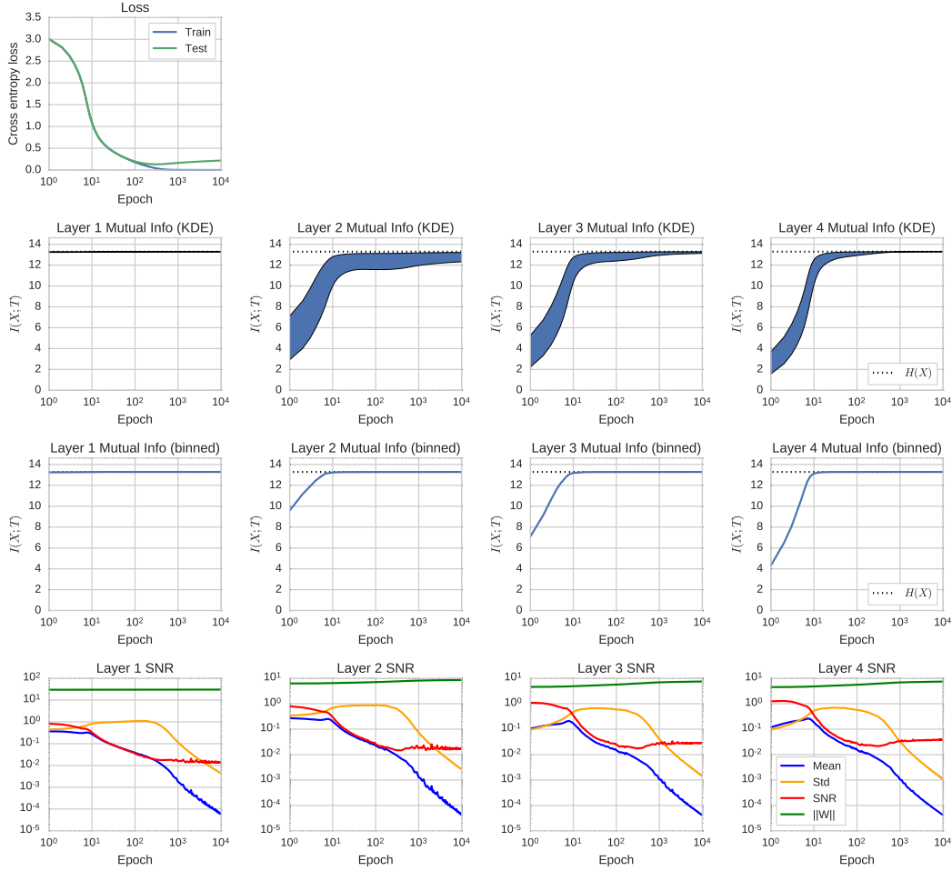
Figure 10: Detailed ReLU activation function results on MNIST. Row 1: Loss over training. Row 2: Upper and lower bounds for the mutual information I(X; T) between the input ( X ) and each layer’s activity ( T ), using the nonparametric KDE estimator (Kolchinsky & Tracey, 2017; Kolchinsky et al., 2017). Dotted line indicates H(X) = \log_2 10000 , the entropy of a uniform distribution over 10,000 testing samples. Row 3: Binning-based estimate of the mutual information I(X; T) , with each neuron’s activity discretized using a bin size of 0.5. Row 4: Gradient SNR and weight norm dynamics. The gradient SNR shows a phase transition during training, and the norm of the weights in each layer increases. Importantly, this phase transition occurs despite a lack of compression in the ReLU network, indicating that noise in SGD updates does not yield compression in this setting.
