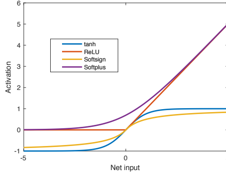
Figure 11: Alternative activation functions.
